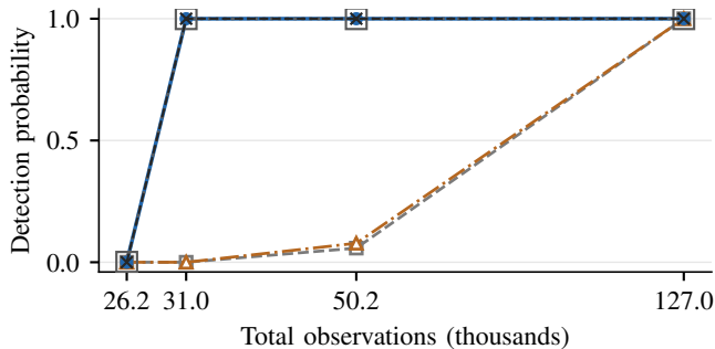
(a) Two balanced categories
