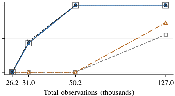
(b) Eight categories with a rare cell
