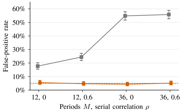
(a) Null: extrapolation with \beta = 2
