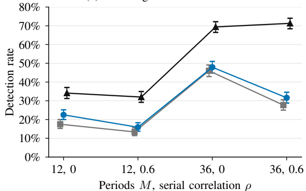
(b) Weak signal: leave-cluster scores
