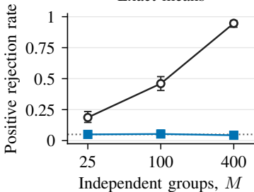
(a) Resampled peers Exact means
