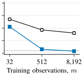
(b) Resampled peers Fitted means
