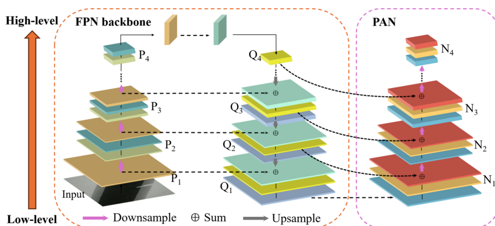
Fig. 9 Hybrid pyramid structure
