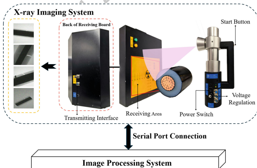
Fig. 2 High-voltage cable NDT equipment
