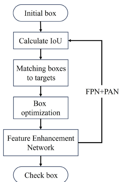
Fig. 8 Flowchart of the IoU-guided box refinement strategy
