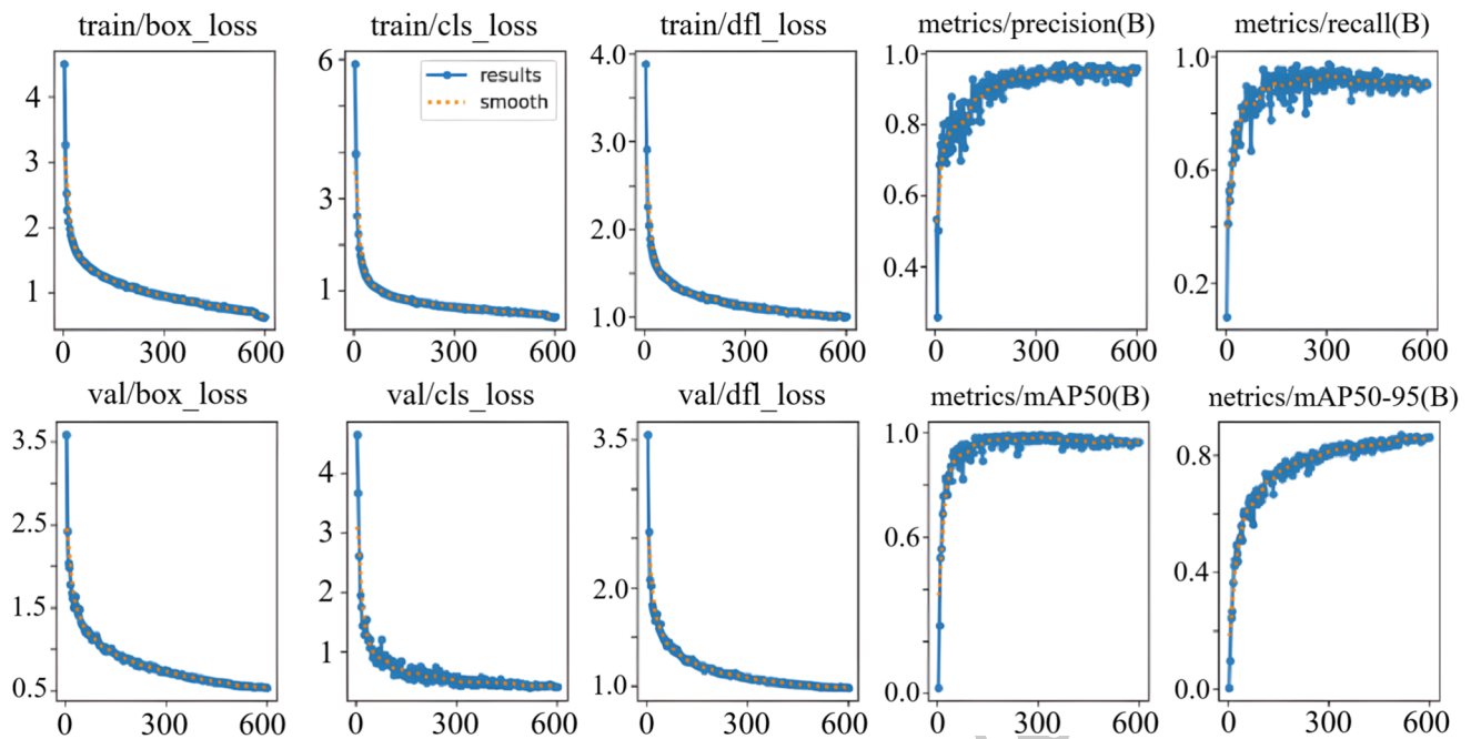
Fig. 11 EMA-YOLOv8 model evaluation index results
