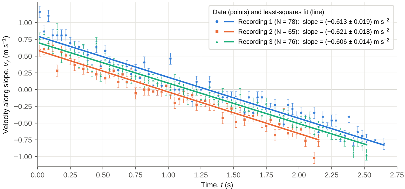
Up-slope velocity v_y vs time for three projectile launches (table tilt \theta = 3.5^\circ )
