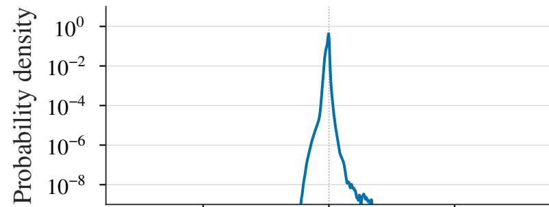
(a) FFN pre-activation
