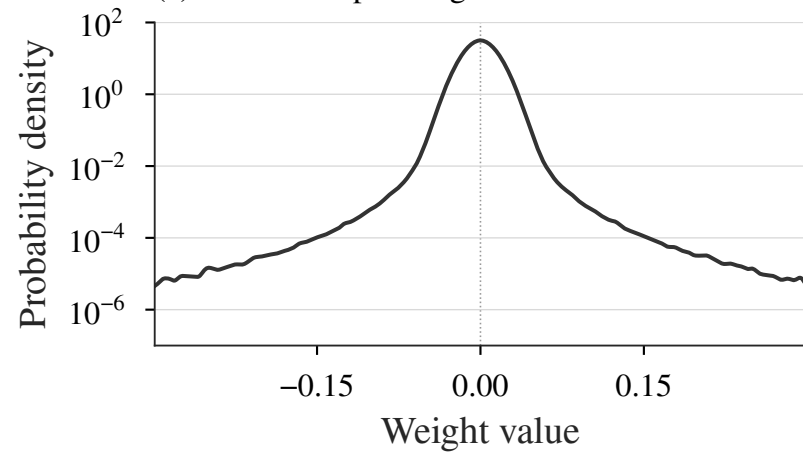
(e) Mamba output weights
