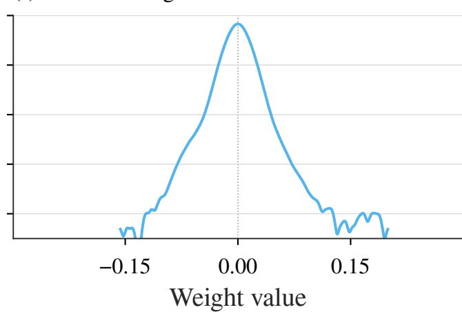
(f) LM head weights
