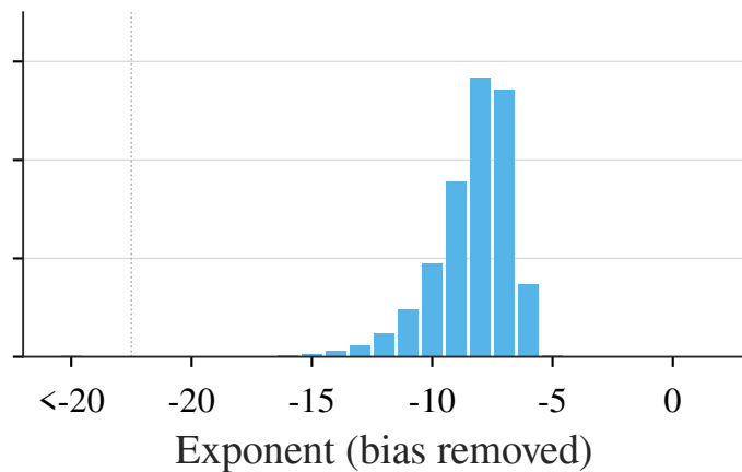
(f) LM head weights
