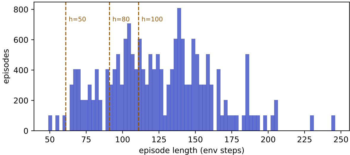
Push-T episode lengths (n=18685, median 123)
