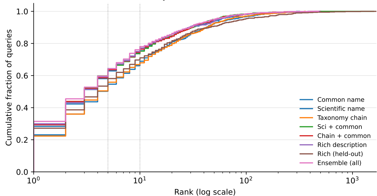
Rank CDF (fraction of queries with first hit \leq rank) — finetuned
