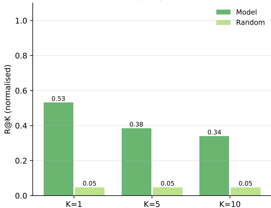
Same-family neighbour recall
