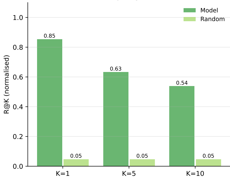
Same-family neighbour recall
