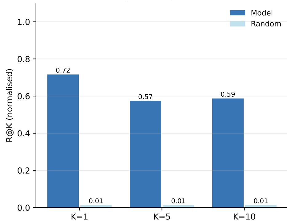
Same-genus neighbour recall
