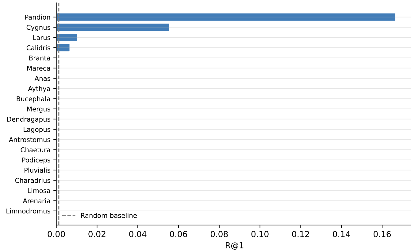
R@1 per genus (top-20 by R@1)
