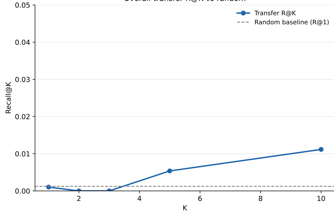
Overall transfer R@K vs random
