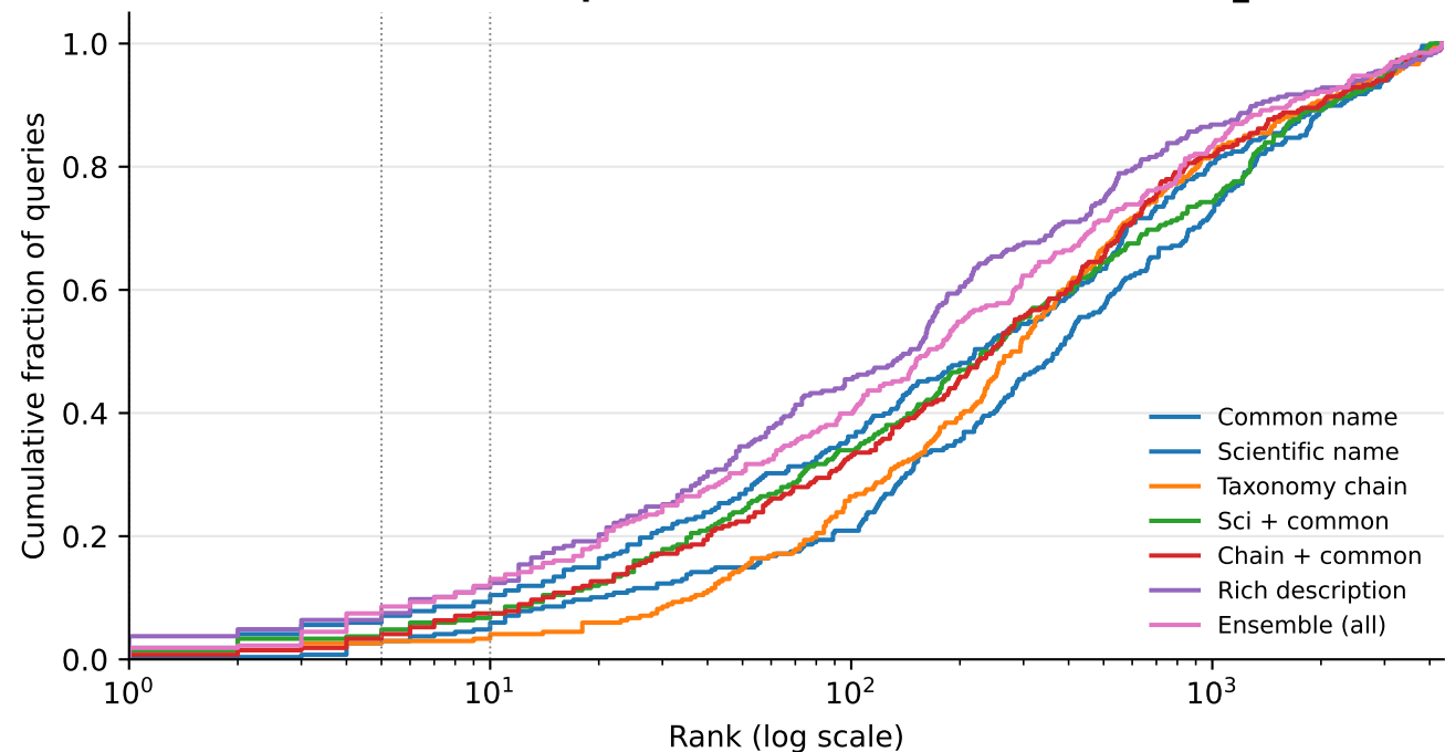
Rank CDF (fraction of queries with first hit \leq rank) — base_zero-shot
