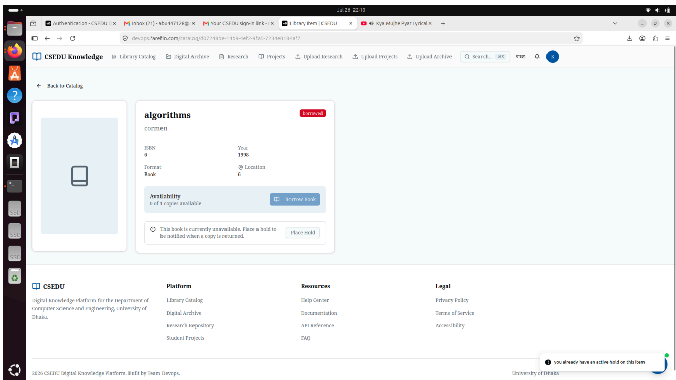
Figure 31 — Place a hold. /catalog/{id} for an unavailable title — Place Hold action
