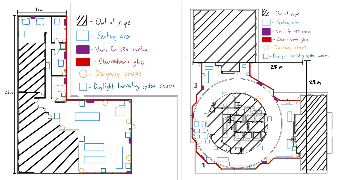
Figure 20. Floor plan of Solution 2 on the 27th (right) and 28th (left) floors.
