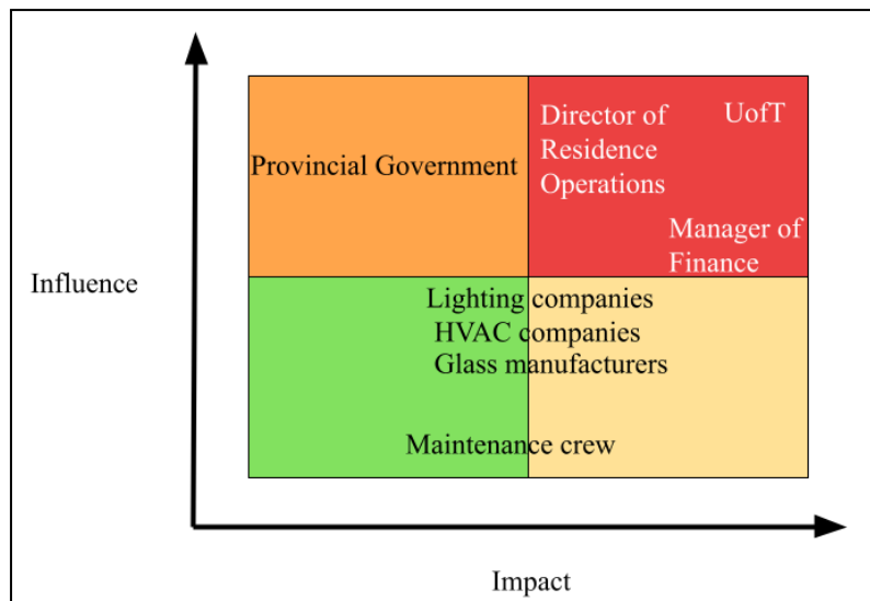
Figure 27. Influence-Impact Graph
