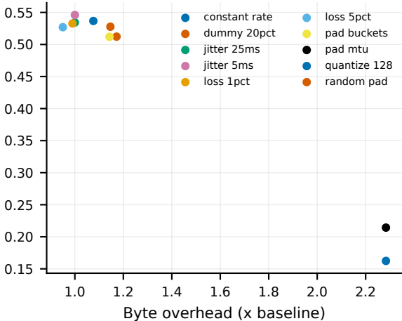
Macro-F1 under defence
