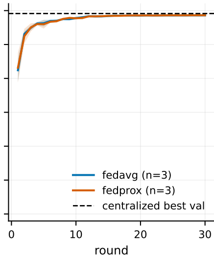
alpha = 1
