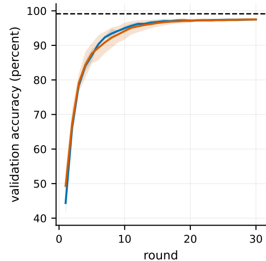
alpha = 0.1
