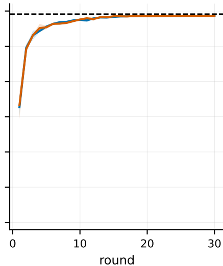
alpha = 0.5
