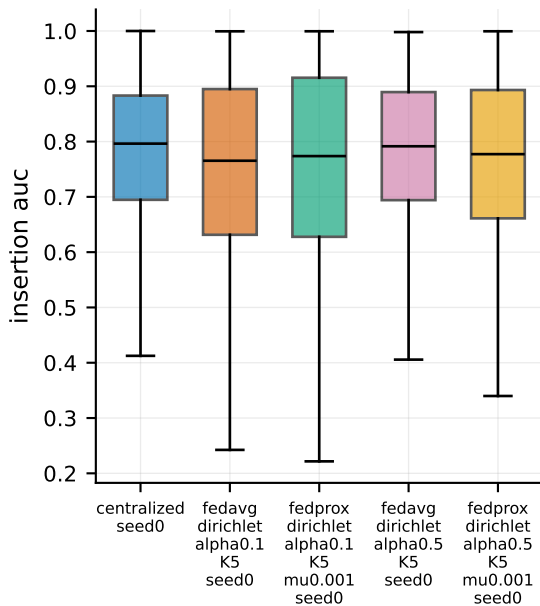
gradcam
