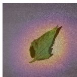
gradcam overlay
