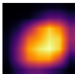
gradcam heatmap
