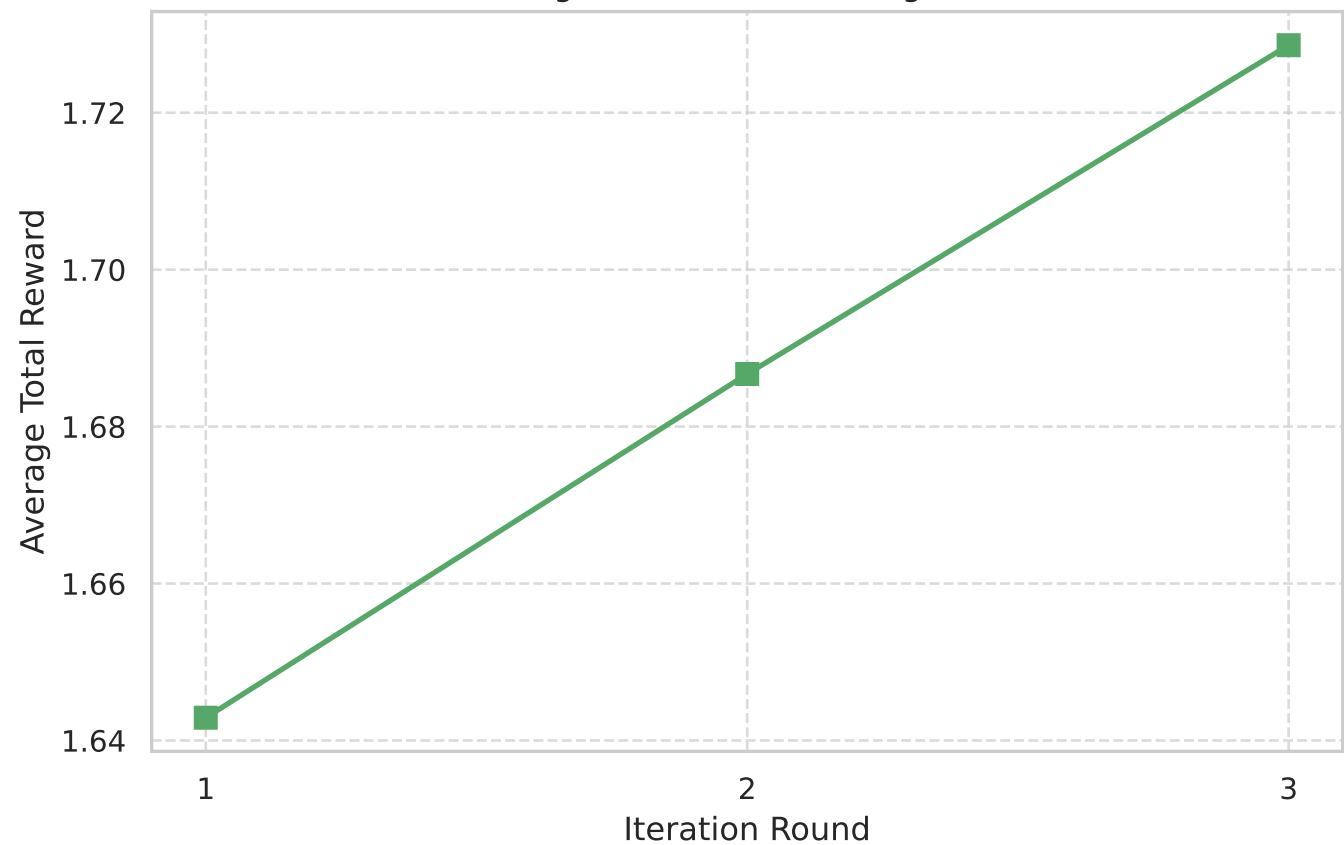
LLM Agent Total Reward Progression
