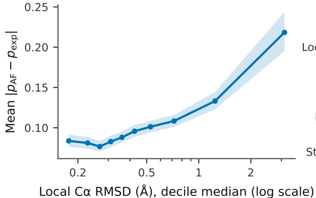
(a) Prediction shift vs. local RMSD
