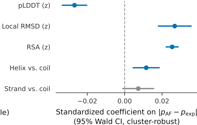
(b) Shift regression coefficients
