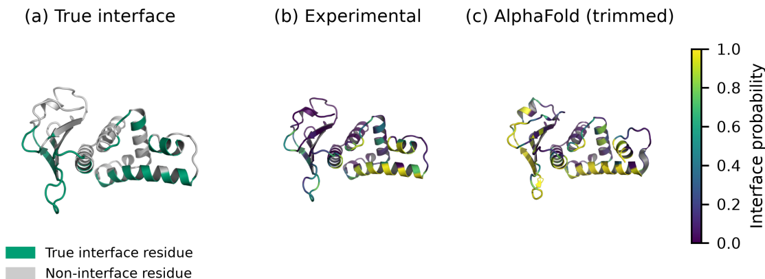
Figure 6: A representative chain (rendered with PyMOL (cartoon representation), not a C \alpha trace; the AlphaFold model in (c) is Kabsch-superposed onto the experimental structure and all three panels share one camera orientation; produced by scripts/render_example_chain.py , see Code and Data Availability). (a) True interface residues (green) vs. non-interface (grey). (b) PeSTo’s per-residue interface probability from the experimental structure (AUPR 0.837 on this chain). (c) PeSTo’s per-residue interface probability from the AlphaFold model trimmed to the same residue range (AUPR 0.806, scored on the same residues as (b)), superposed onto the experimental frame for comparison only (the underlying coordinates, and hence the prediction, come from the AlphaFold model).
