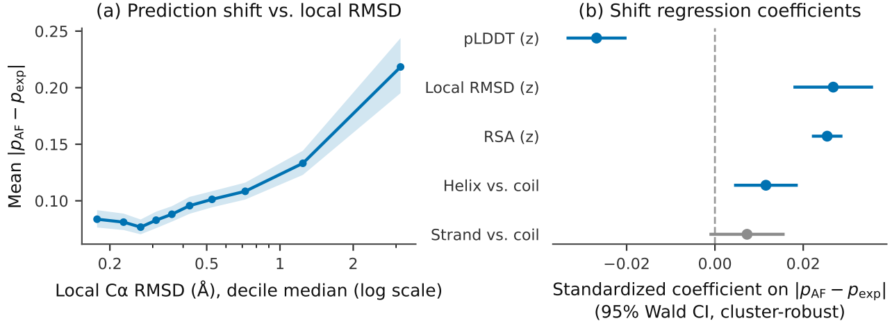
Figure 5: (a) Mean absolute prediction shift in each decile of local C\alpha RMSD (equal numbers of residues per decile), plotted at the decile’s median local RMSD on a log scale, with chain-resampled 95% CIs. (b) Standardized coefficients (95% Wald CI, cluster-robust) from the per-residue shift regression; grey markers did not reach p < 0.05 .
