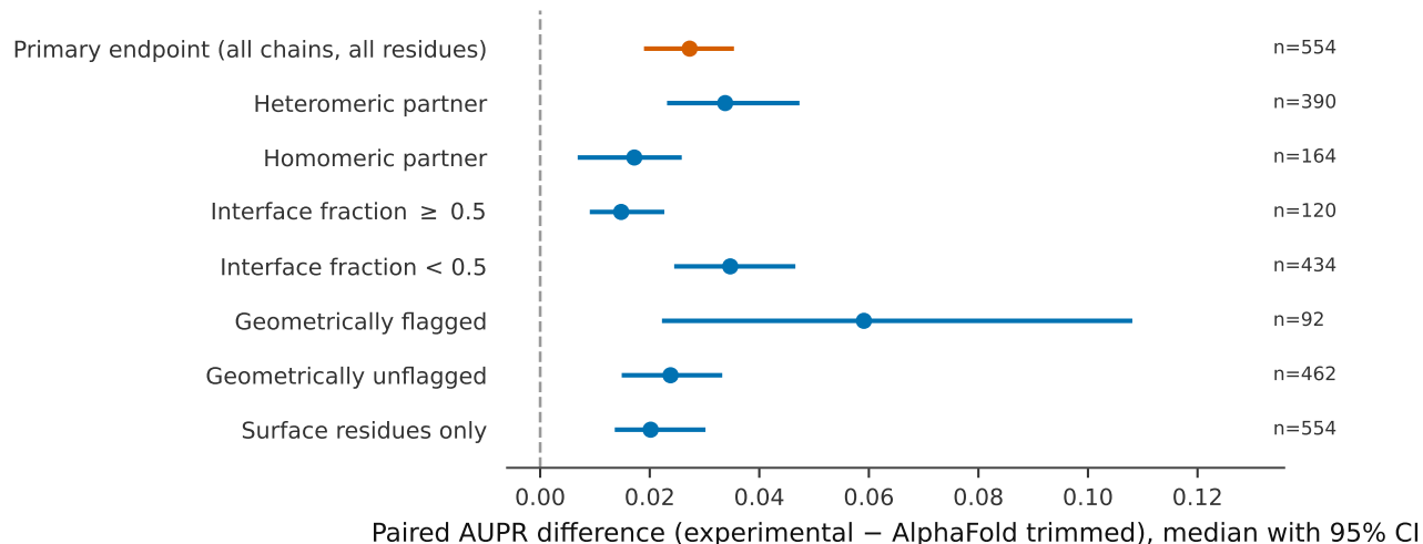
Figure 3: Paired AUPR difference (median, 95% chain-resampled bootstrap CI) for the primary endpoint and the subgroups of the four pre-specified descriptive splits. The all-residues subgroup is identical to the primary endpoint and is shown once. All intervals lie on the same side of zero.
