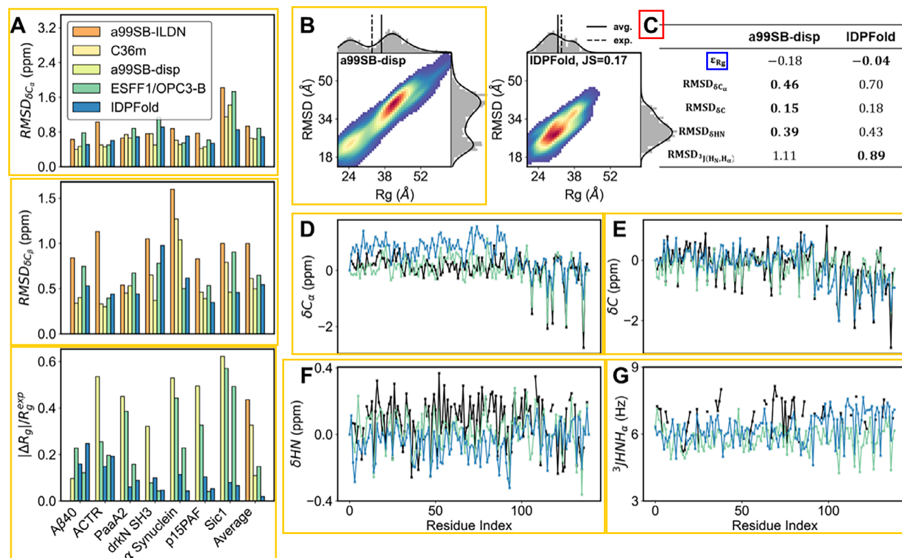
Figure 4. Comparison between the performance of IDPFold and that of all-atom MD simulations with different force fields. A) Accuracy of IDPFold in estimating local features ( \delta C_{\alpha} , \delta C_{\beta} , chemical shifts) and global feature Rg compared to MD simulations. B) Rg-RMSD distribution of IDPFold-generated ensemble compared to MD simulation with a99SB-disp on \alpha Synuclein. C) Errors between generated ensembles and experimental observations for a99SB-disp and IDPFold on \alpha Synuclein. D–G) Local Features including \delta C_{\alpha} chemical shifts (D), \delta C_{\beta} chemical shifts (E), HN chemical shifts (F) and ^3J(HN, H_{\alpha}) (G) of IDPFold generated ensembles and MD simulation with a99SB-disp on \alpha Synuclein. 300 conformations are sampled for each system.
