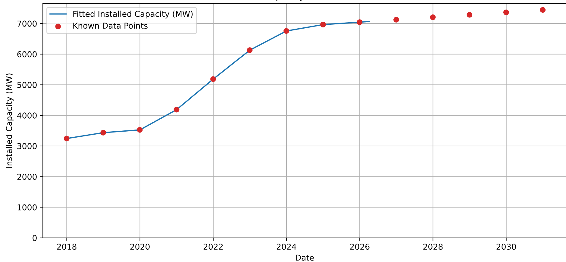
Installed Onshore Wind Capacity NL: Fitted vs Known Data Points
