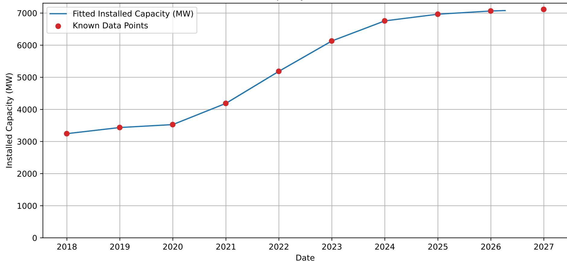
Installed Offshore Wind Capacity NL: Fitted vs Known Data Points
