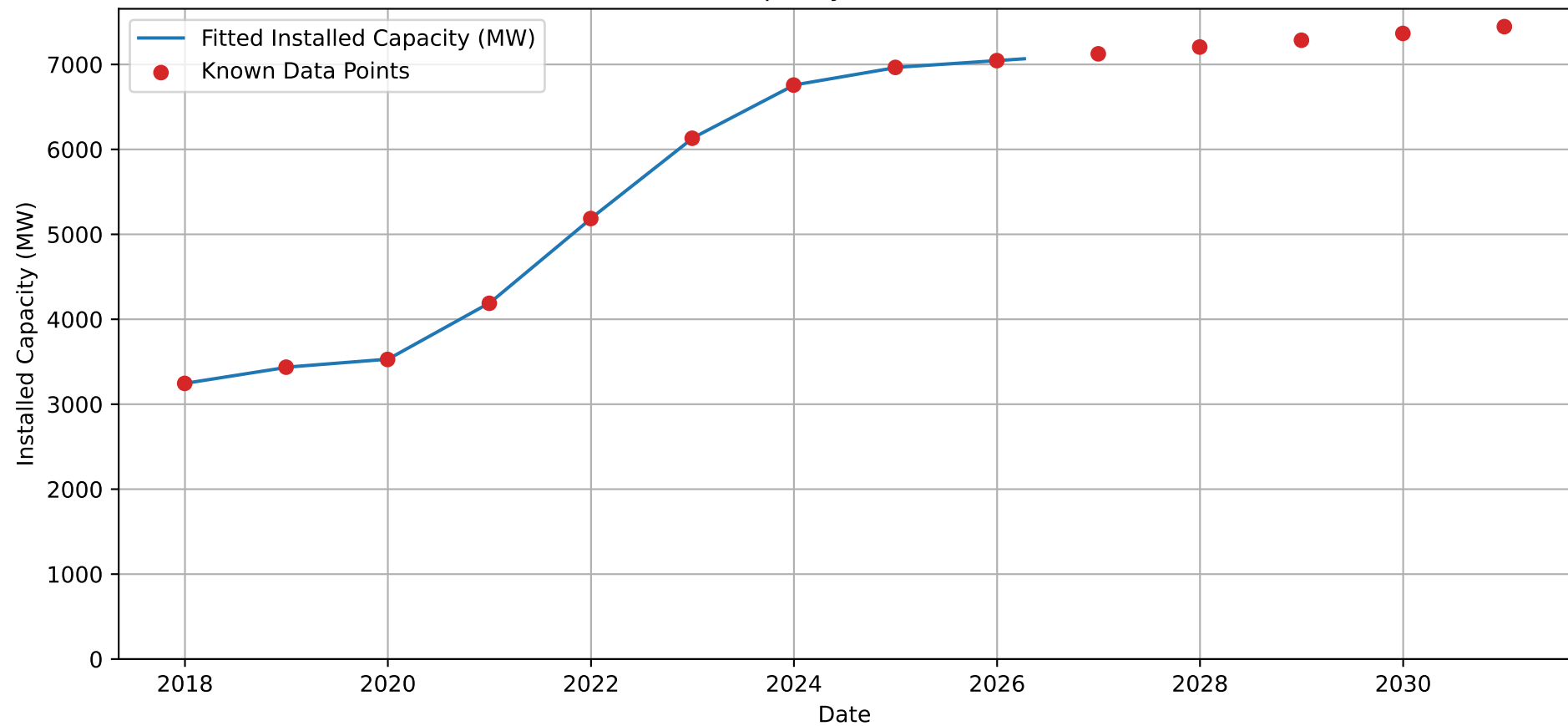
Installed Wind Onshore Capacity NL: Fitted vs Known Data Points
