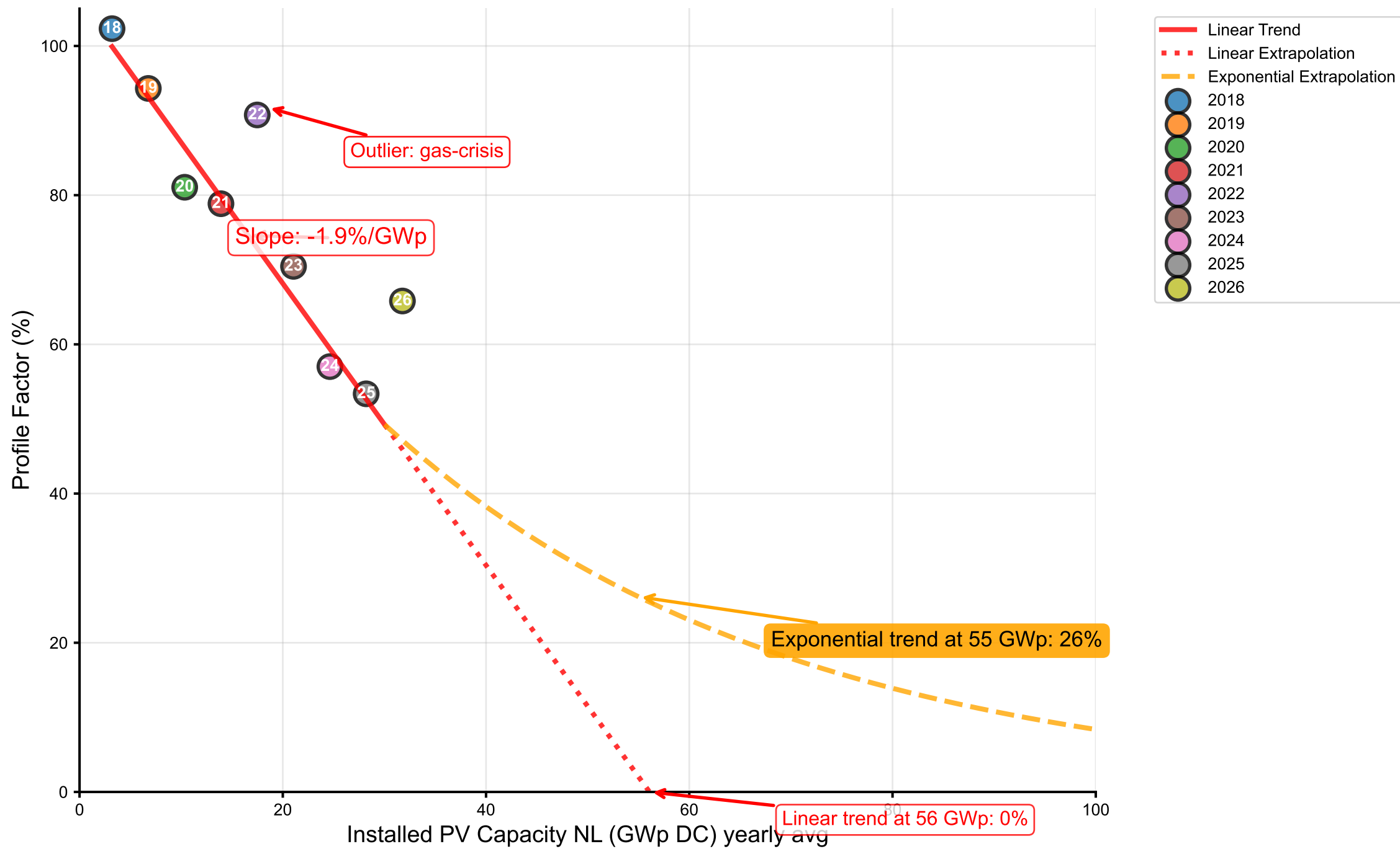
PV Profile Factor vs Installed Capacity Solar PV in Netherlands Each point represents year avg installed capacity vs yearly PV profile factor
