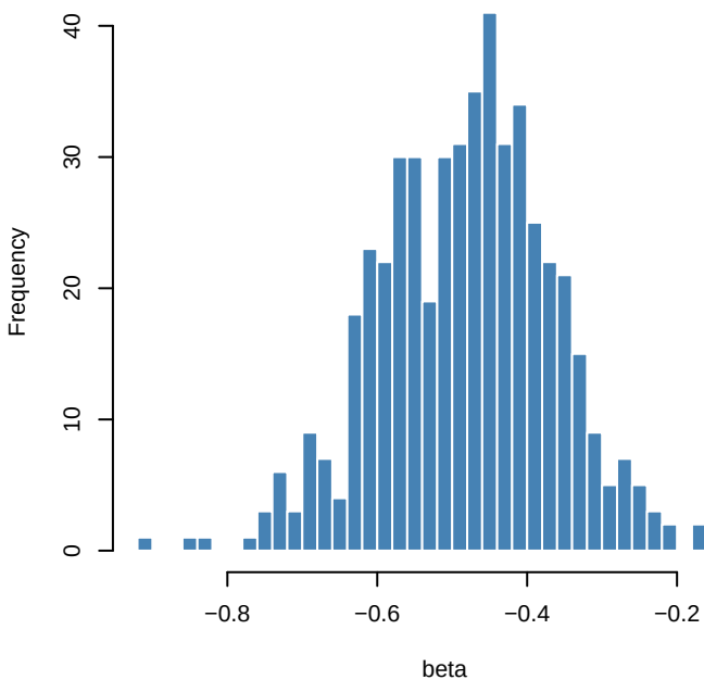
Null scenario (true_effect=0): opposite signs 67.6%
