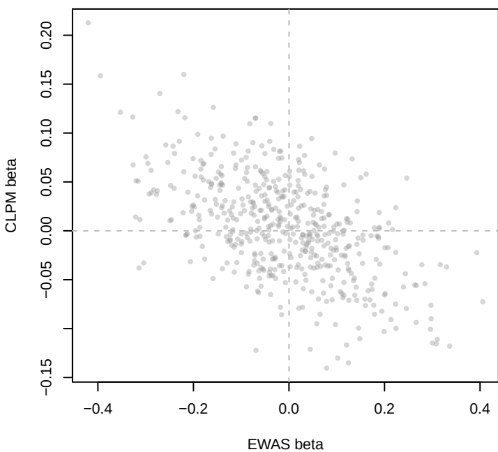
Null scenario (true_effect=0): opposite signs 67.6%
