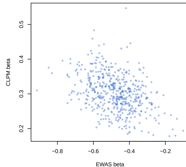
EWAS vs CLPM (opposite signs: 100.0%)
