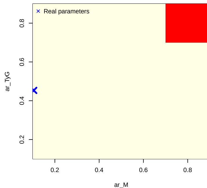
Proportion opposite signs (true_effect = 0.3)
