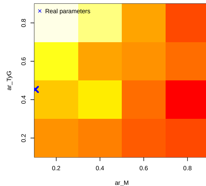
Proportion opposite signs (true_effect = 0, null)
