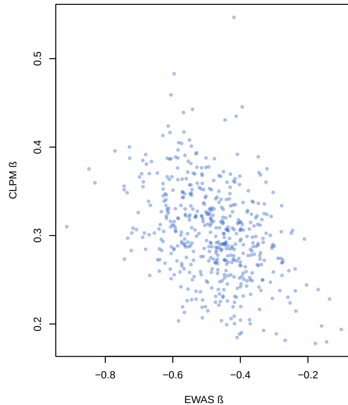
EWAS vs CLPM (.....: 100.0%)
