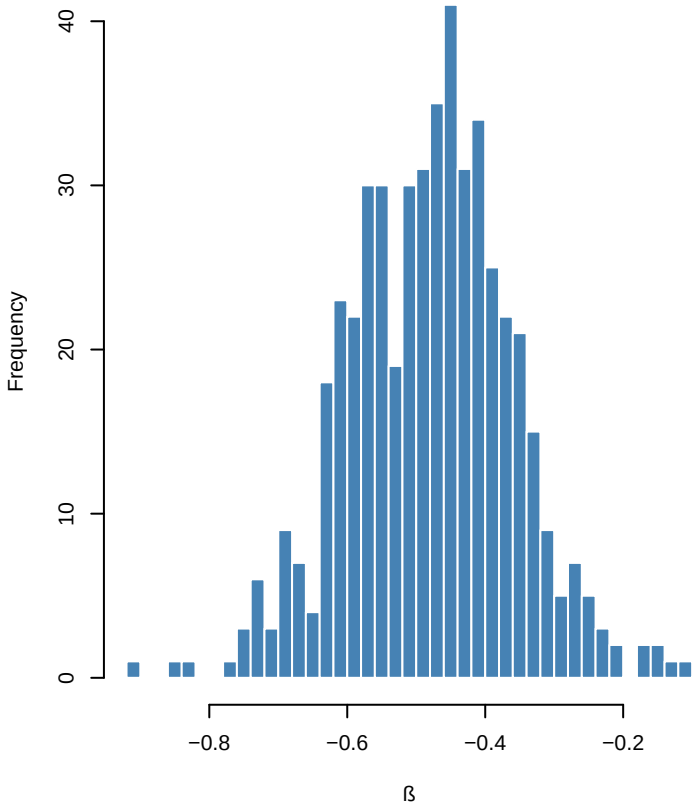
EWAS \beta (..ar_M=0.10, ar_TyG=0.45)
