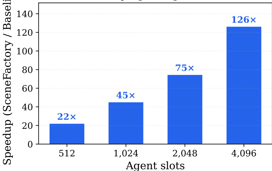
SceneFactory Speedup over Baseline
