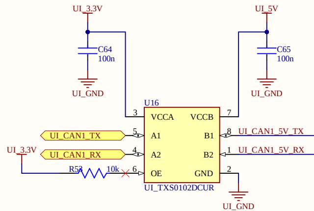
UserInterface_CAN_LogicShifter
