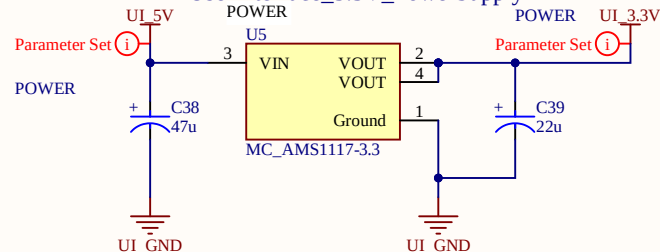
UserInterface_3.3V_PowerSupply
