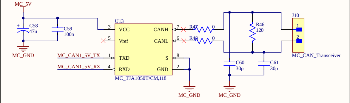
MotionCore_CAN_Transceiver
