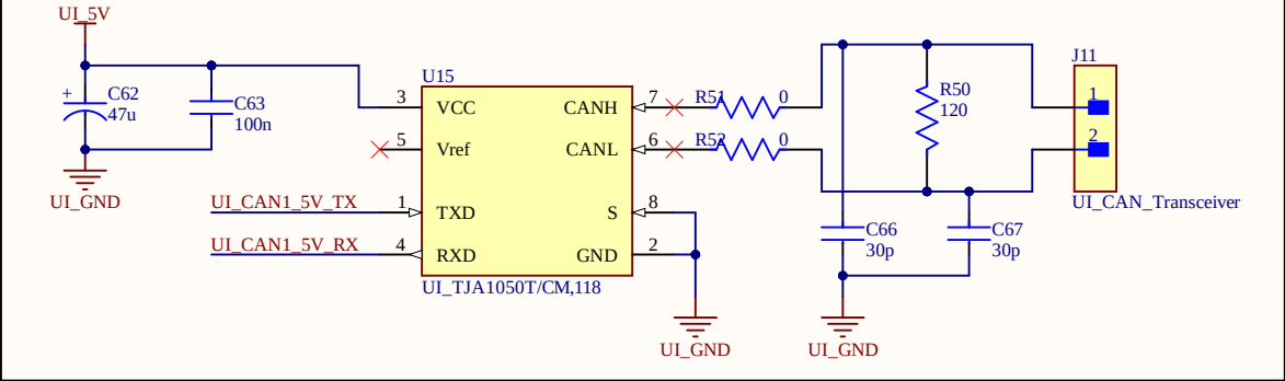
UserInterface_CAN_Transceiver
