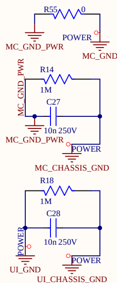
Ground net connection
