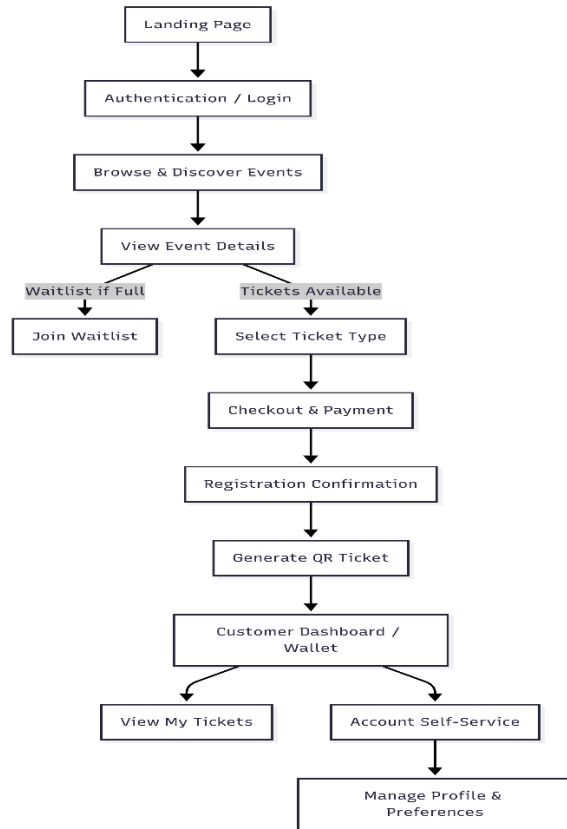
Customer User Flow Diagram
