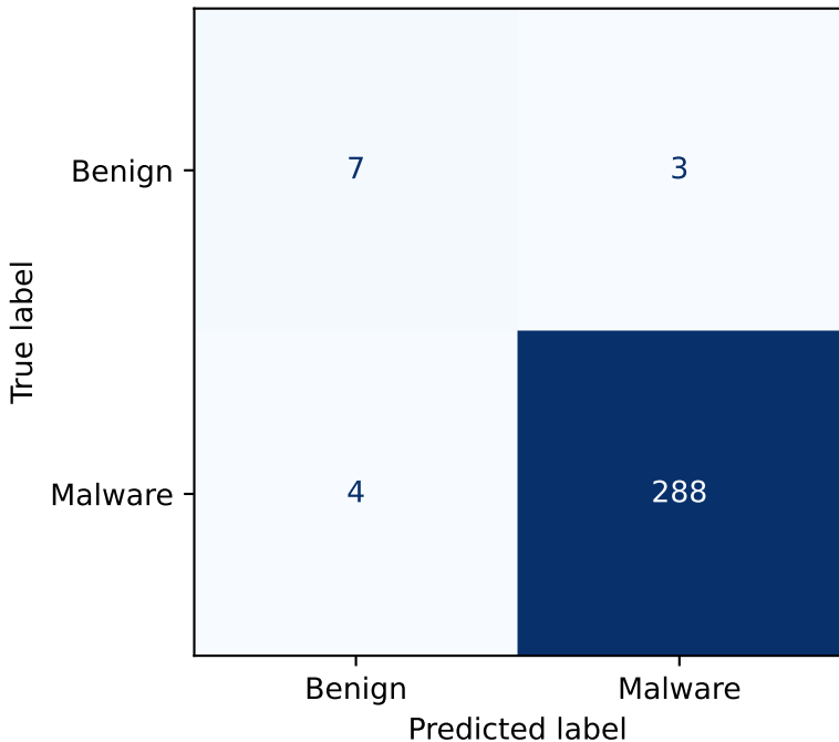
hydra Confusion Matrix
