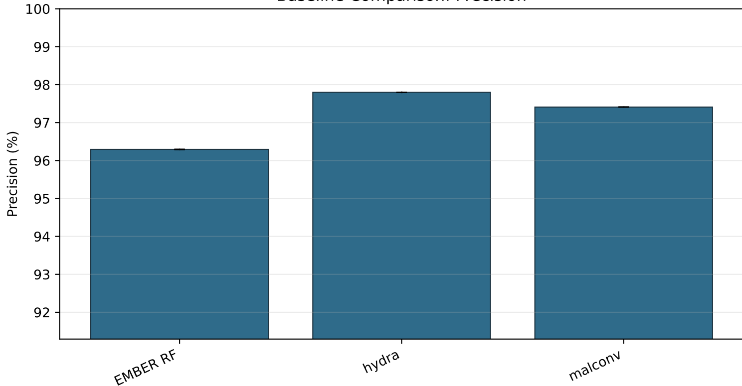
Baseline Comparison: Precision
