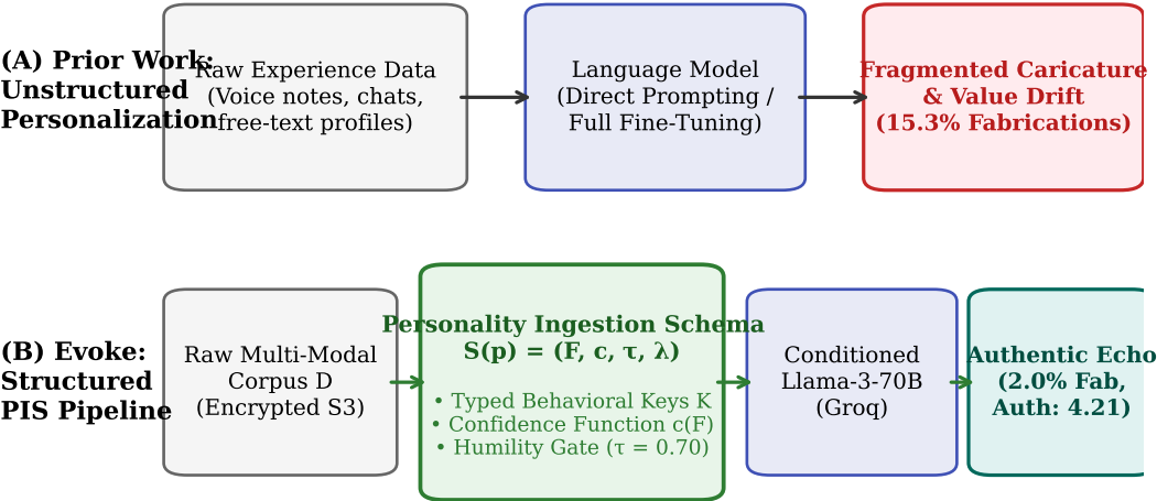
Fig. 1. Conceptual contrast: Prior Unstructured Approaches vs. Evoke Structured PIS
