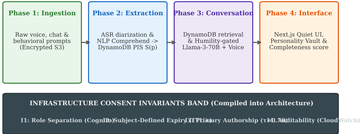
Fig. 4. Four-phase pipeline with underlying Consent Invariants Band (I1-I4)
