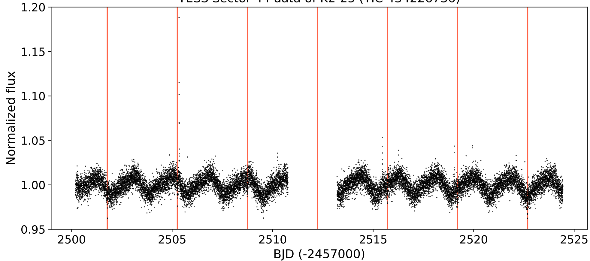
TESS Sector 44 data of K2-25 (TIC 434226736)
