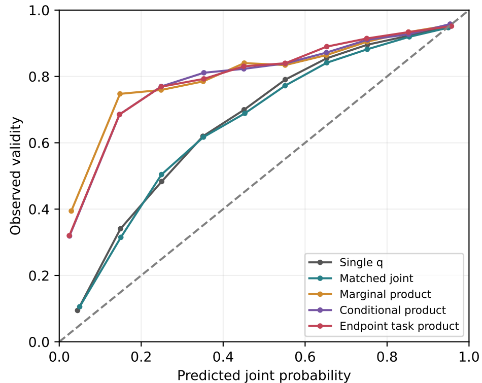
Calibration and candidate risk-coverage | natural unfiltered pools
