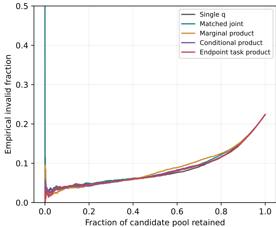
Calibration and candidate risk-coverage | natural unfiltered pools
