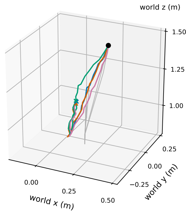
All K4 paths; grey = 3 recorded references
