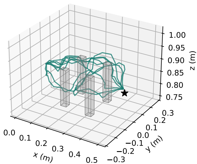
R1 / open: valid 8/8, modes 7
