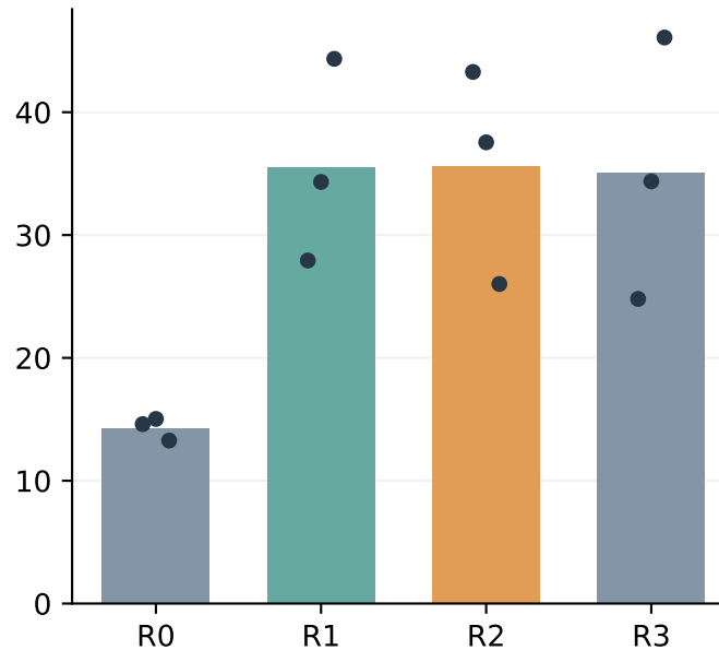
Shared-mode recall (%)
