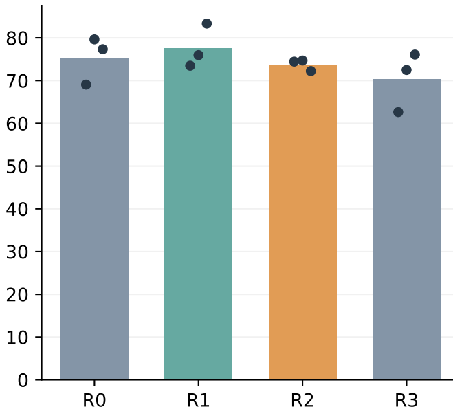
Candidate validity (%)
