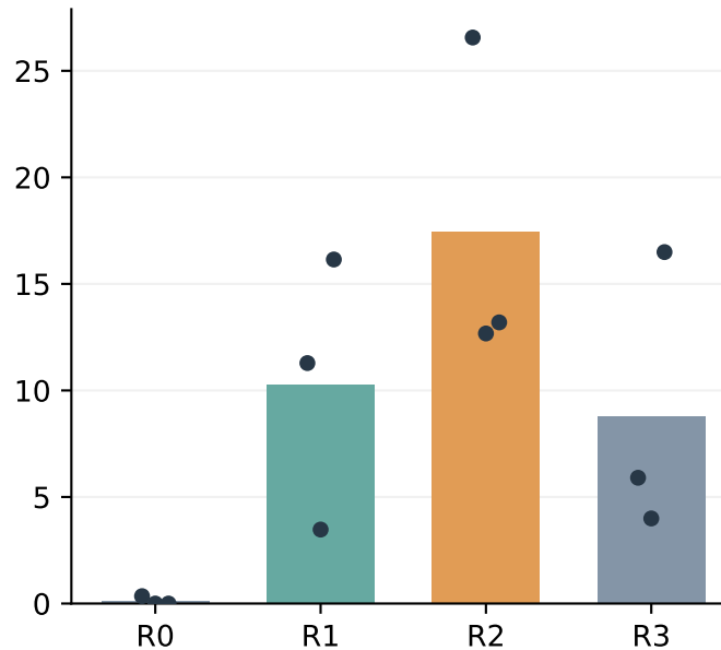
Opened-mode recall (%)
