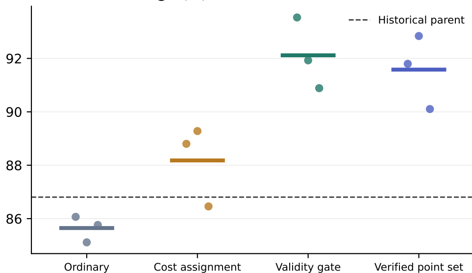
Known-mode recall @8 (%)
