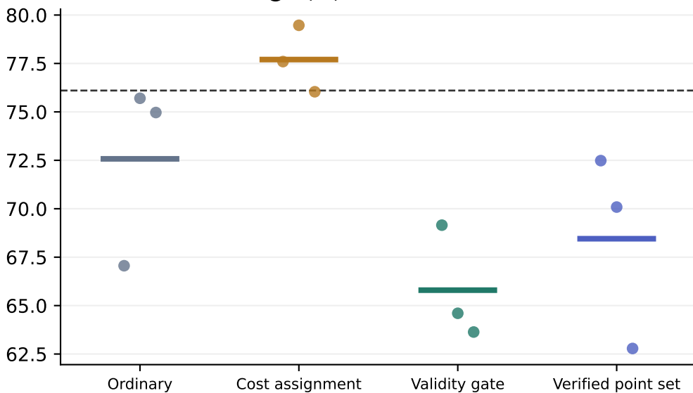
Known-mode recall @8 (%)
