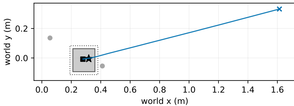
obstacle_reach_272102_target1 / whole4 finite 1/4; 3D TipValid 0/4
