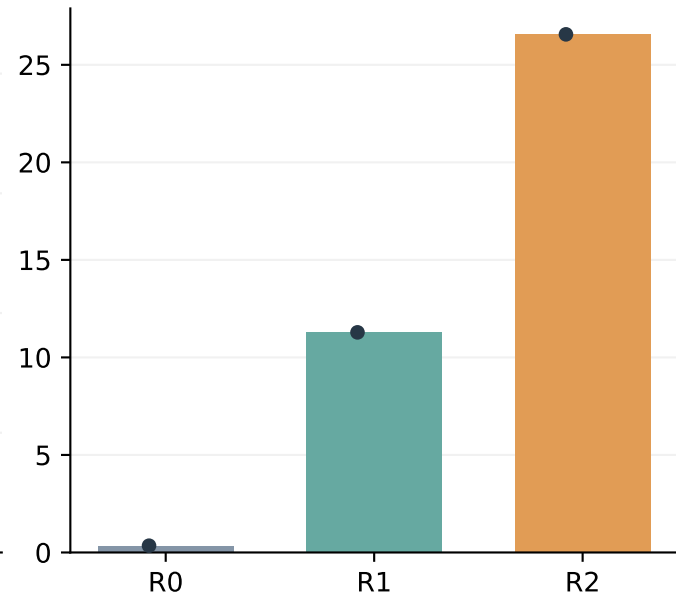
Opened-mode recall (%)
