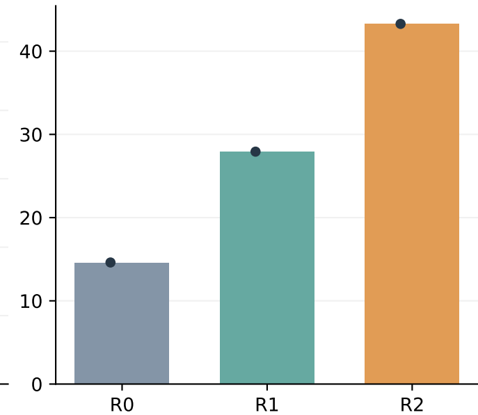
Shared-mode recall (%)
