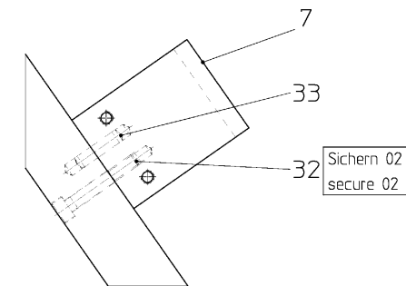
Detail 2 (1:1)
