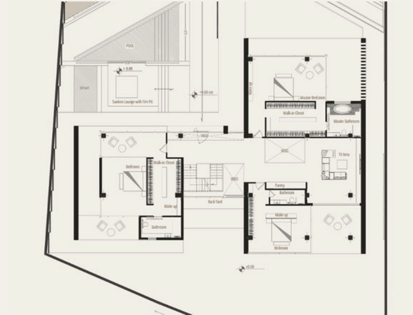
First-floor plan. Private rooms held within the two upper frames.
