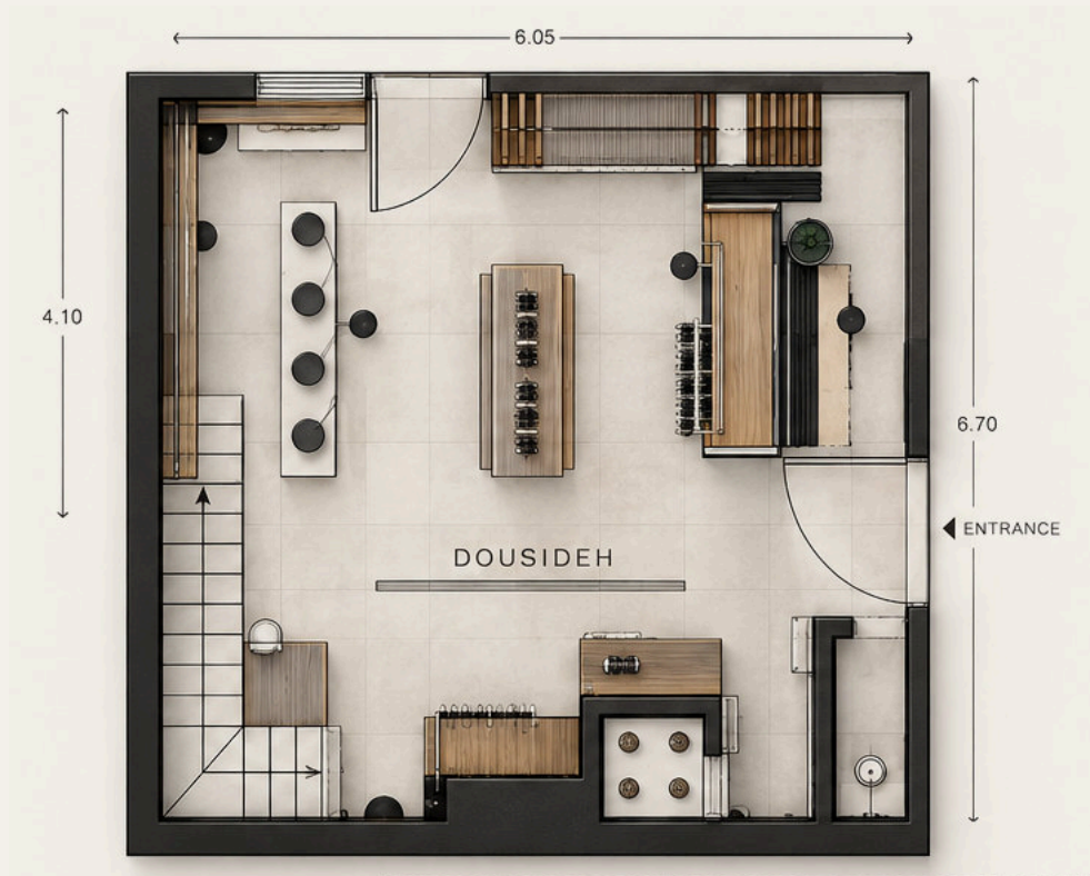
Key plan. Display tables, wall joinery, counter and stair.
