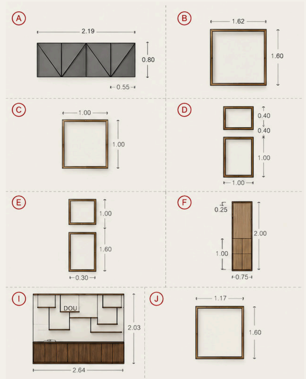
Joinery elevations. Keyed to the plan and dimensioned for fabrication.
