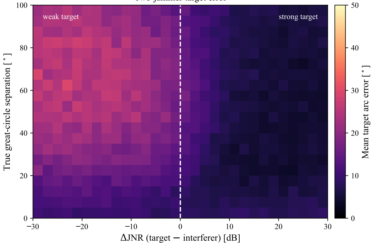
Two-jammer target error
