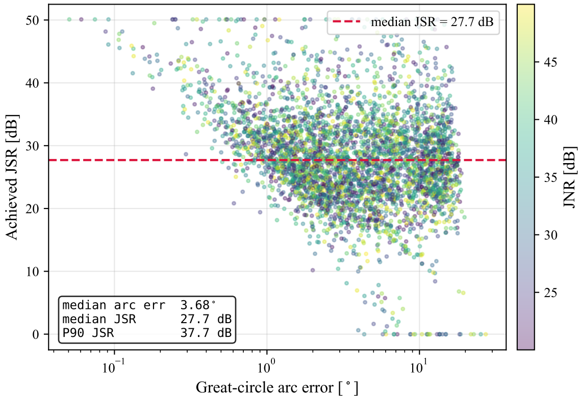
Single-jammer suppression vs estimation error
